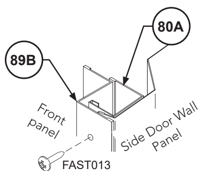
SECTION VIEW
